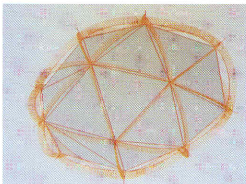
Figure 5: A Convex Polyhedron with Quadric Wires : \rho = 0.4
