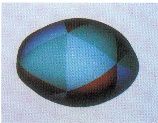
Figure 6: A C^1 Smooth Polyhedron with Quintic Algebraic Patches : \rho = 0.4
