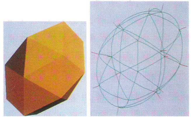
Figure 2: A Convex Polyhedron and its C^1 Conic Wireframe
