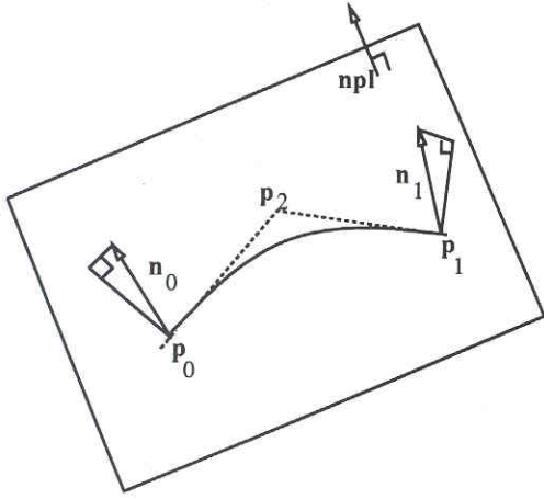
Figure 1: Computation of a Conic Curve
