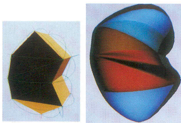
Figure 9: Smoothing the Non-Convex Polyhedron with Quintic Algebraic Patches
