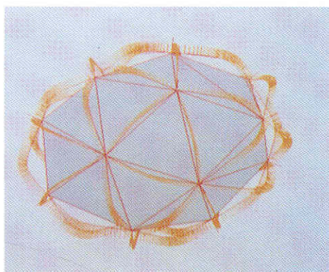
Figure 7: A Convex Polyhedron with Quadric Wires : \rho = 0.75
