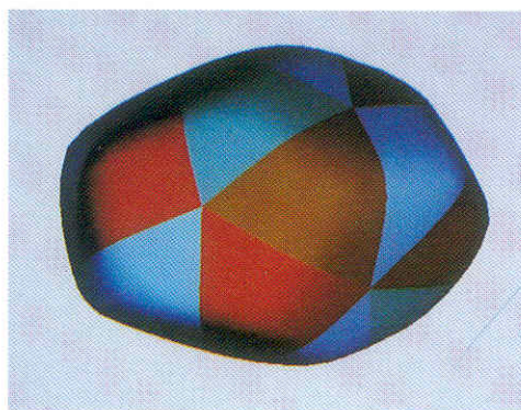
Figure 8: A C^1 Smooth Polyhedron with Quintic Algebraic Patches : \rho = 0.75
