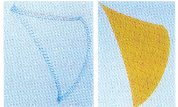
Figure 3: A Quadric Triangle and its C^1 Patch
