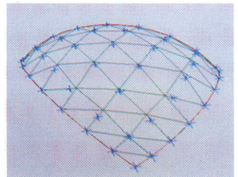
Figure 4: A Triangulation for Display and Additional (+) Points for Shape Control
