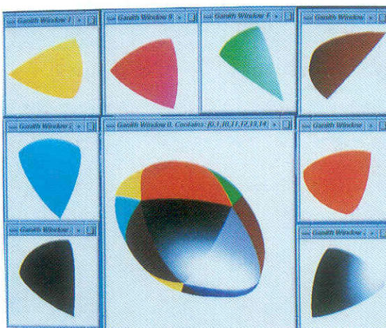
Figure 10: A Polyhedron Smoothed in the SHASTRA Distributed and Collaborative Geometric Design Environment
